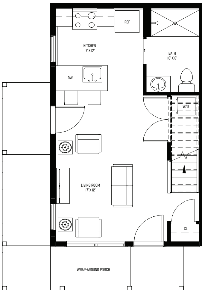
1ST FLOOR
