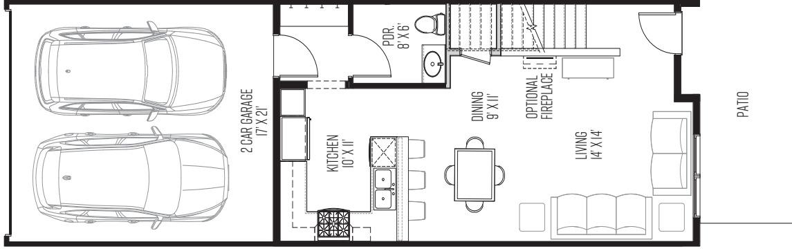
1ST FLOOR
